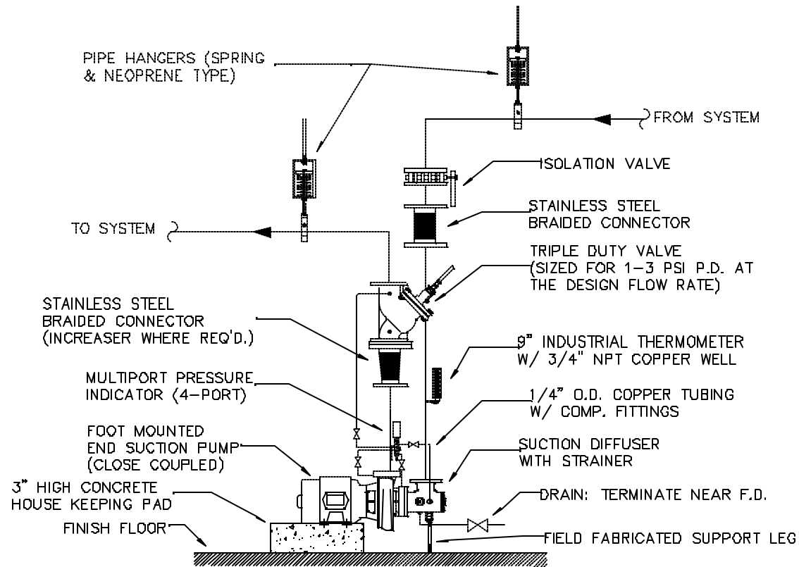
4 END SUCTION PUMP DETAIL - (FOOT MOUNTED ON HOUSEKEEPING PAD) NOT TO SCALE
