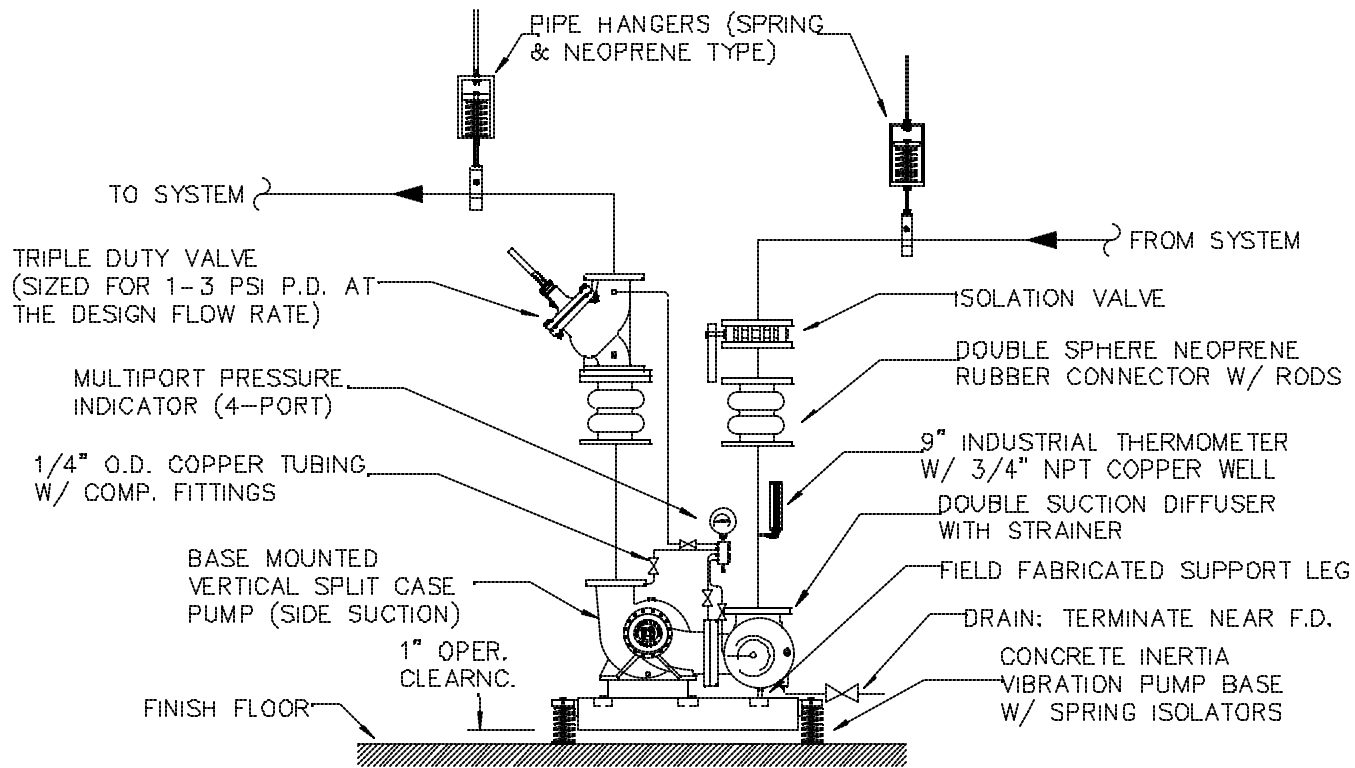
4 VERTICAL SPLIT CASE (SIDE SUCTION) PUMP DETAIL - (BASE MOUNTED ON A CONCRETE INERTIA PAD) NOT TO SCALE
